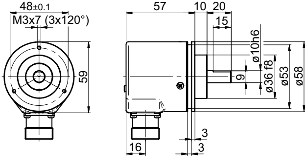
GXP5W - clamping flange and connector M23
